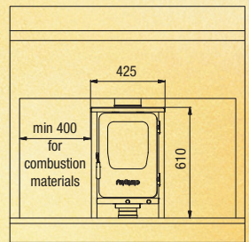
Limiting dimensions of surround and opening
